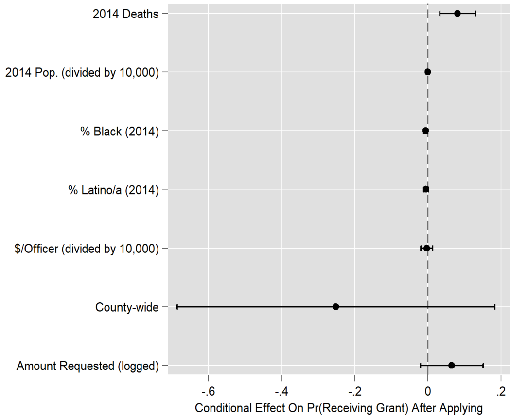
Figure 5.2 Marginal effects of variables on Pr(Received | Applied)
